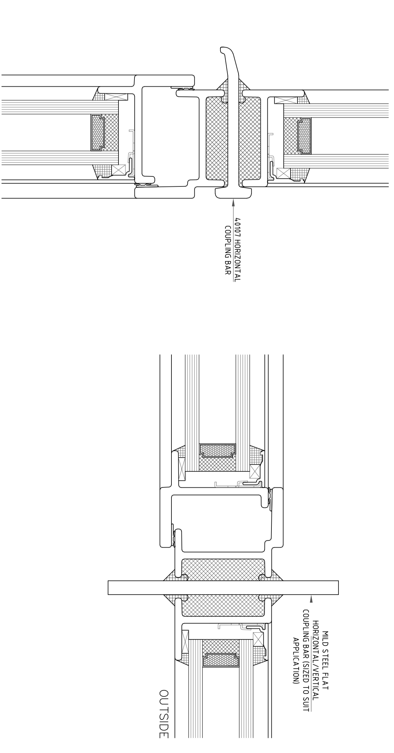
TYPICAL COUPLING DETAILS
