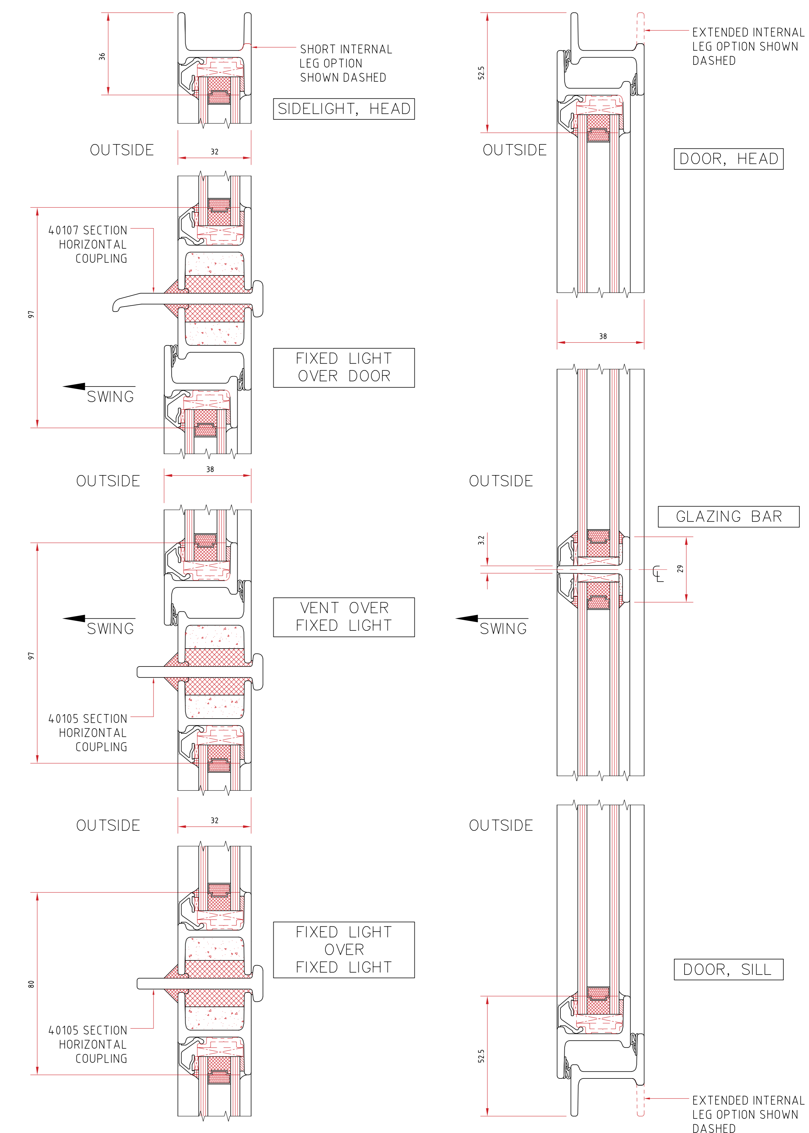
TYPICAL DOUBLE DOOR WITH TOP-LIGHT AND SIDE-LIGHTS
