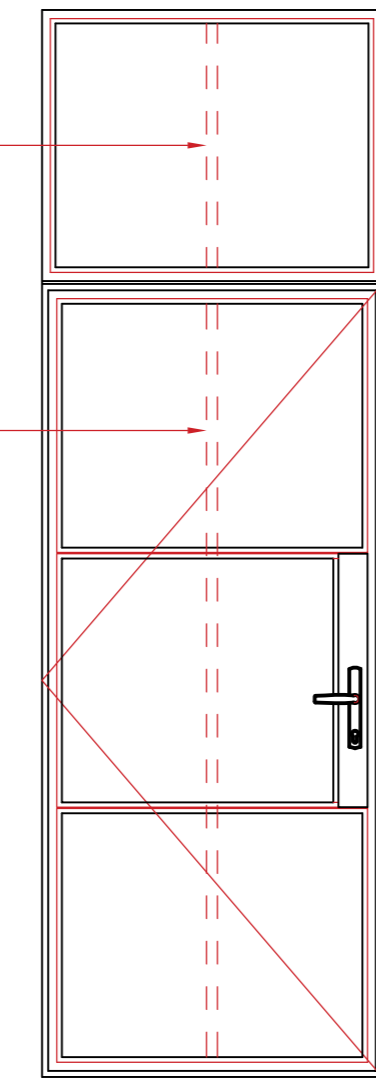
TYPICAL SINGLE DOOR WITH TOP-LIGHT
