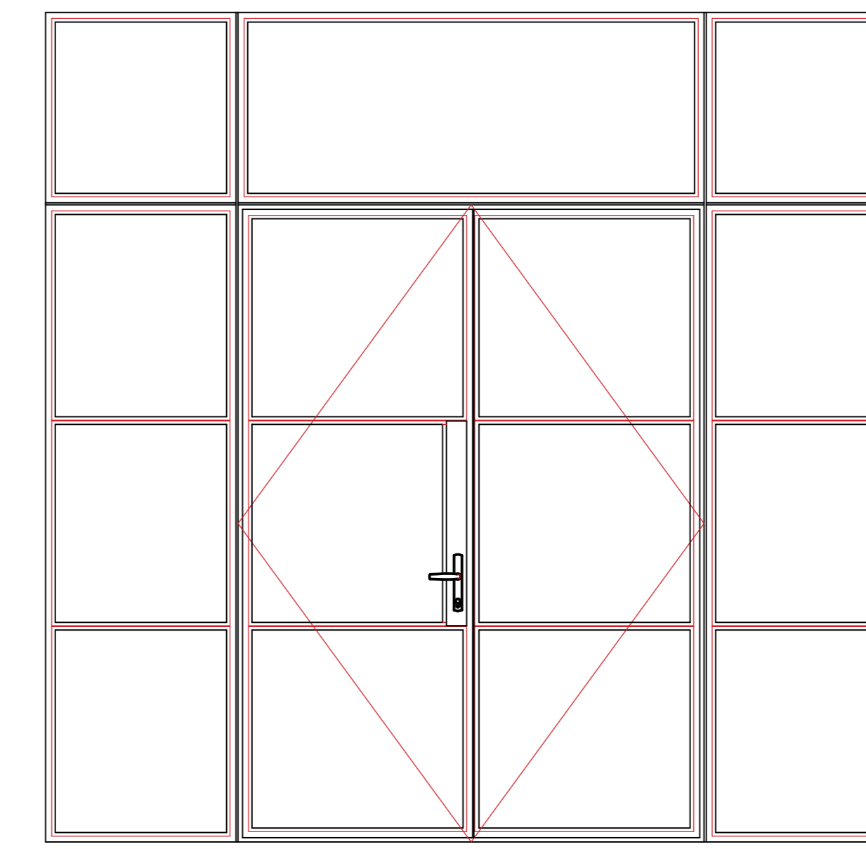
TYPICAL DOUBLE DOOR WITH TOP-LIGHT AND SIDE-LIGHTS
