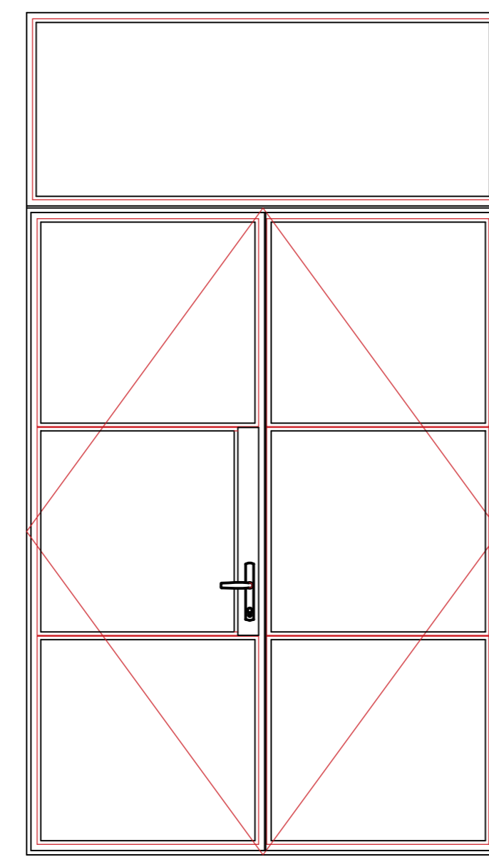
TYPICAL DOUBLE DOOR WITH TOP-LIGHT
