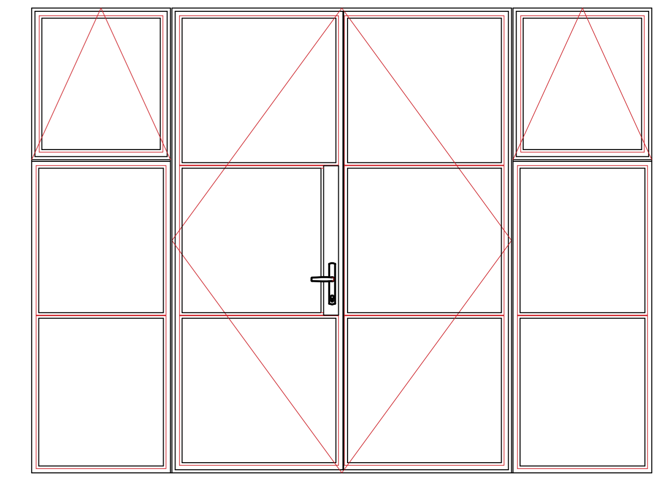
TYPICAL DOUBLE DOOR WITH SIDE-LIGHT AND VENTILATORS
