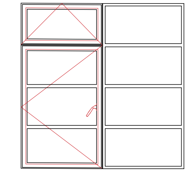
COUPLED ASSEMBLY, EXAMPLE
