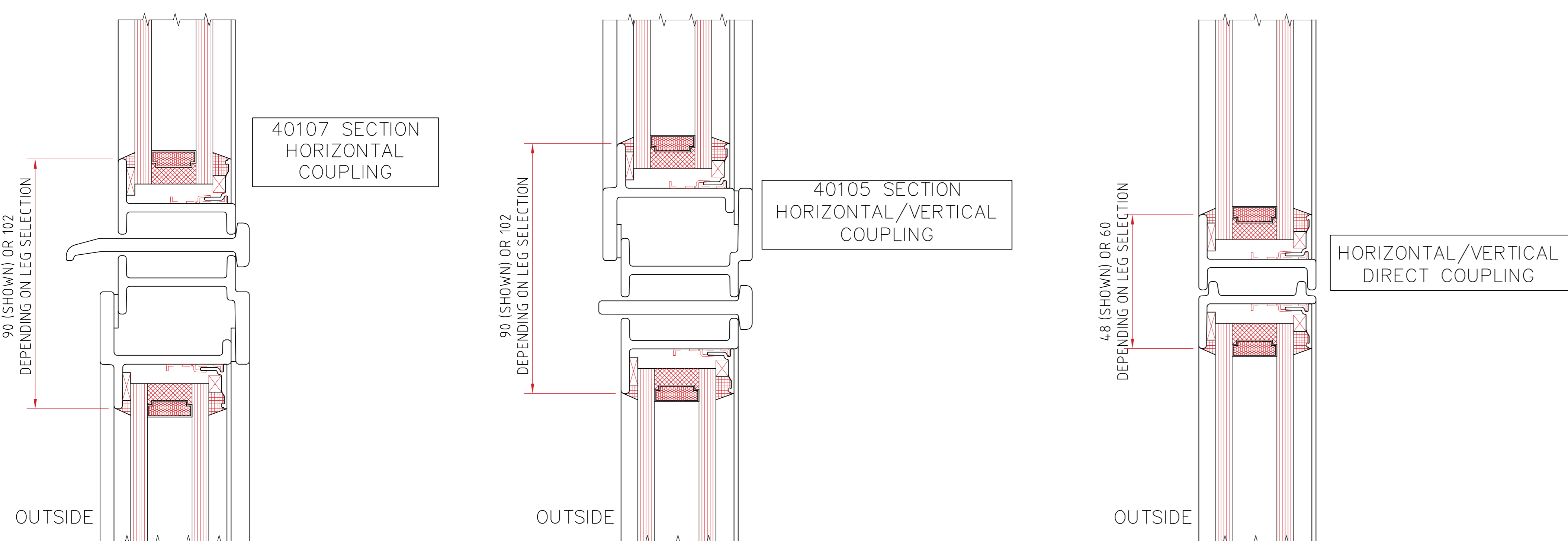
TYPICAL COUPLING DETAILS
